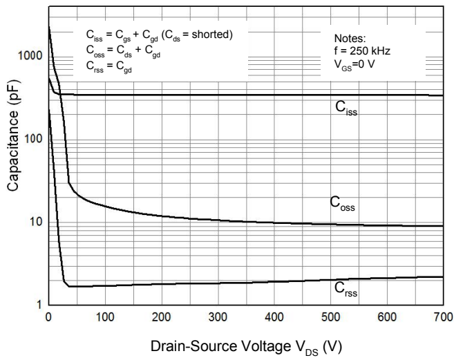
Figure 7. Capacitance Characteristics
