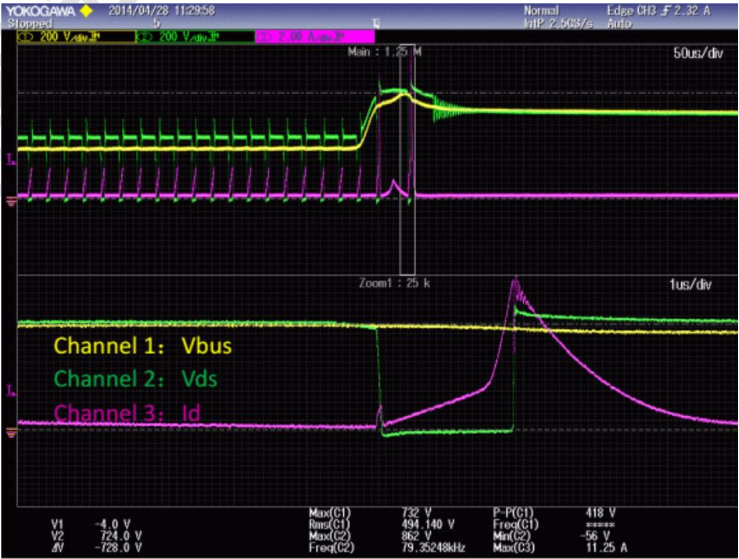
整改前 surge 电流波形 (220Vac,1300V/90° )
